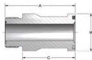
CODE 62 ORFS THREAD
