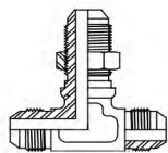
Air-Way Steel MJIC Bulkhead Union Branch Tee
