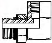
Air-Way MSAE ORING - FNPT 90 Deg Elbow
