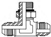
Air-Way Steel MJIC - MSAE ADJ Branch Tee
