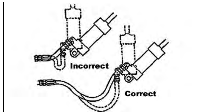
Fig.8 Provide adequate hose length to allow for movement of mechanisms. System design should provide sufficient hose length to prevent strain on connections at extreme extension and to prevent kinking of hose at any point throughout the entire range of motion. Either tensile strain or kinking can cause premature failure of hose/tube assemblies and connectors.
