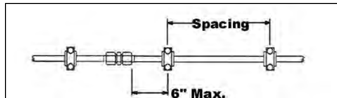
Fig.2 Use proper clamping to reduce strain due to vibration. See Table A for recommended clamp spacing. Final tightening of hose/tube connections should be completed before tightening of supports and clamps.
